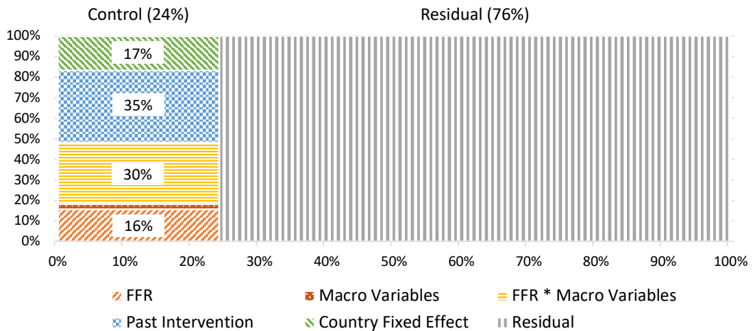
Figure 2: Variance Decomposition for Counter-Intervention
